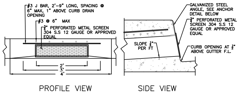
CURB INLET DETAIL
