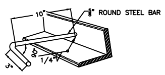
DETAIL OF ANCHOR
